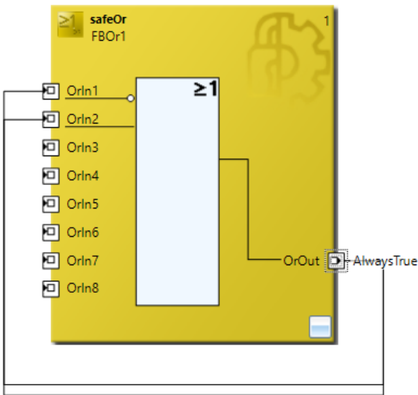
No higher resolution available. Preparing_a_C0001401B_for_TwinSAFE_Project_OrOut.png (436 × 405 pixels, file size: 36 KB, MIME type: image/png)
