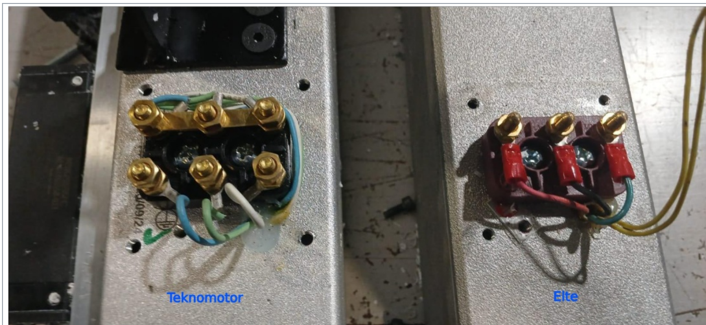
Wiring differences - Wire as Star configuration
